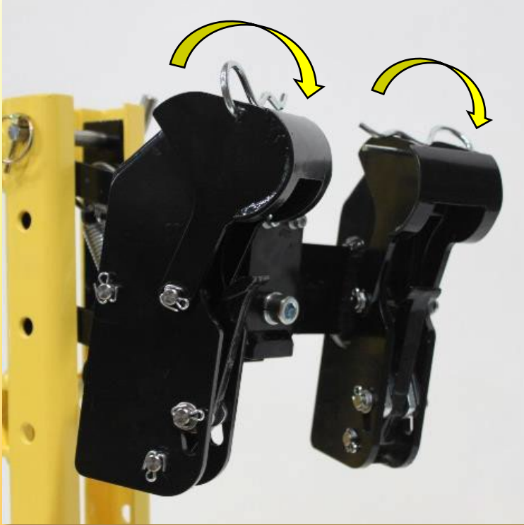
EG2L Clamp with Fiber Drum Guard engaged
