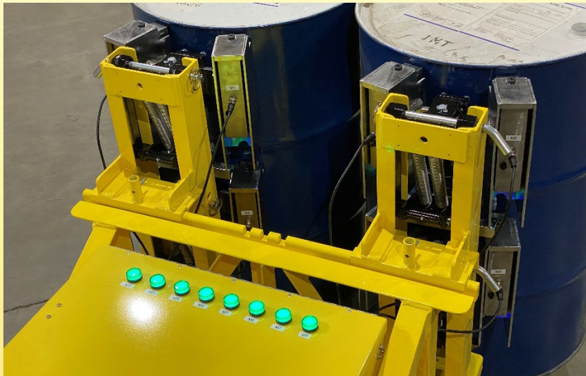
EG4M8DC2-F showing 8 magnets
