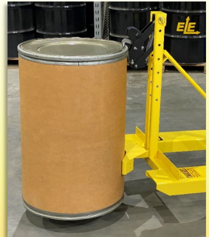
EG1SCM-F w/ Fiber Drum
